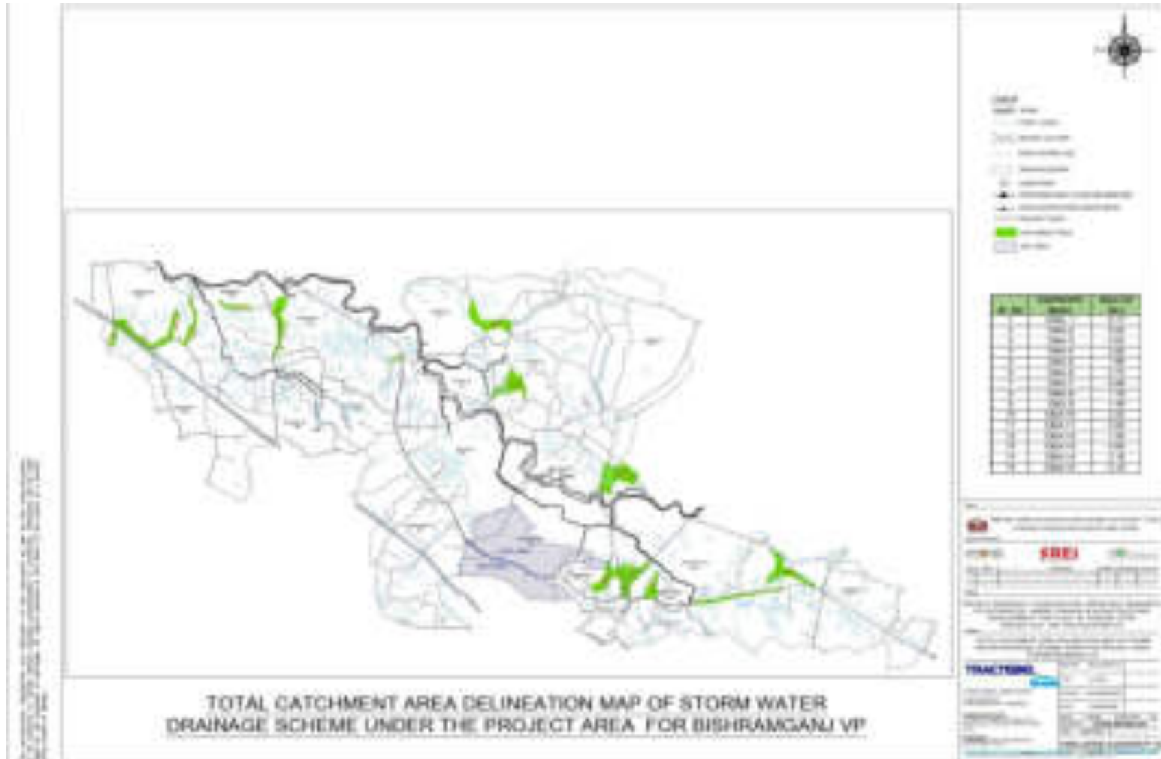
Figure 21: Total Catchment area Delineation map of Storm Water Drainage for Bishramganj
