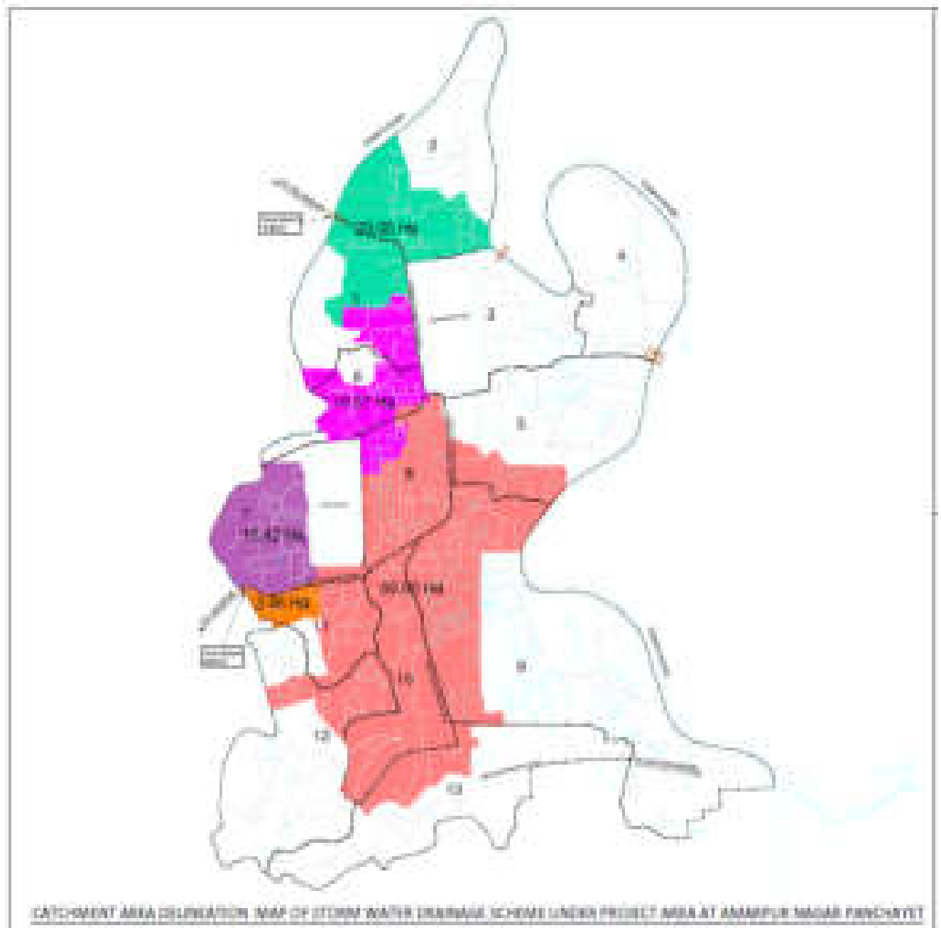
Figure 16: Catchment area delineation map of storm water drainage scheme under project area at Amarpur Nagar Panchayet
