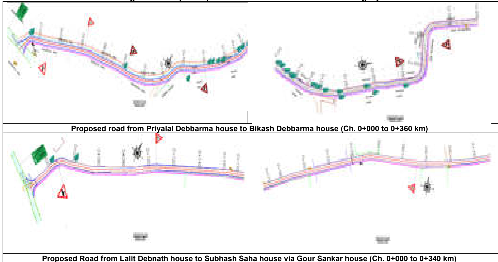
Figure 18: Proposed plan and Profile of the Roads- Bishramganj
