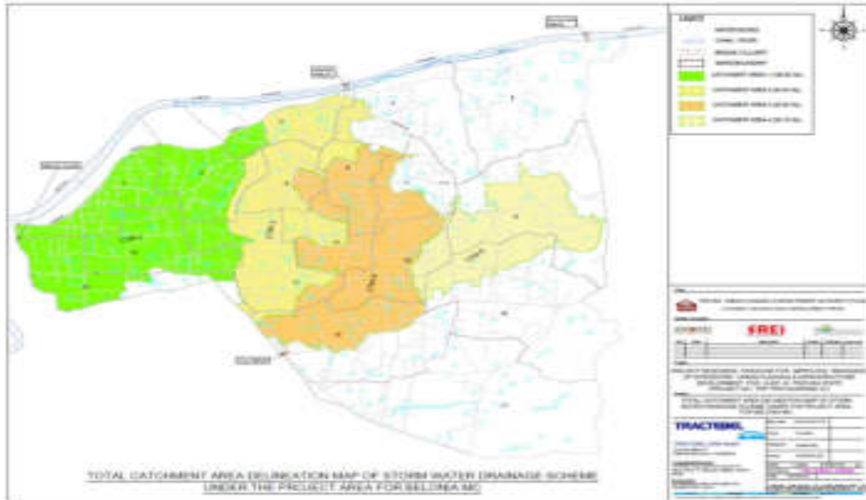
Figure 31: Total Catchment Area Delineation Map of Storm Water Drainage Scheme Under the Project Area For Belonia MC
