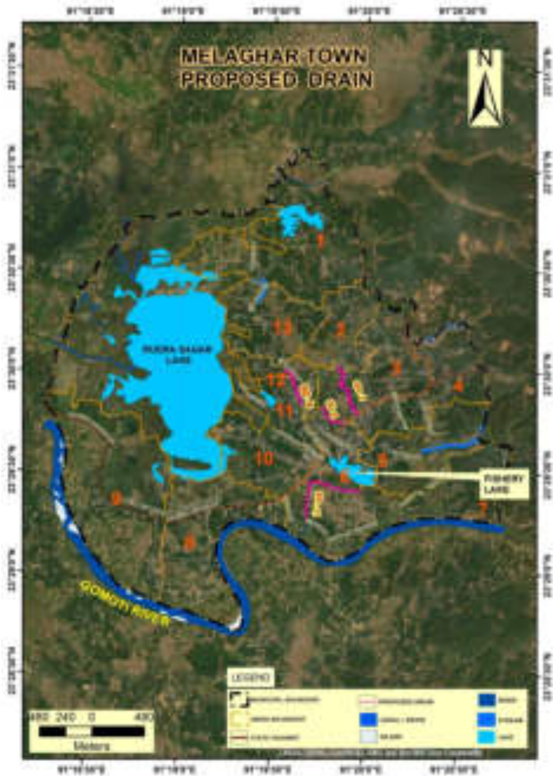
Figure 25: Proposed Drainage components in Melaghar on google earth
