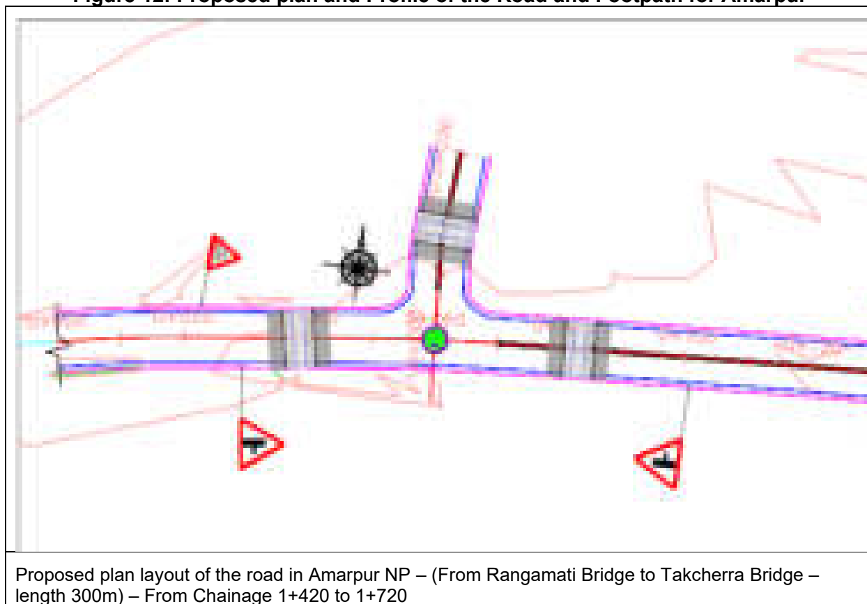
Figure 12: Proposed plan and Profile of the Road and Footpath for Amarpur
