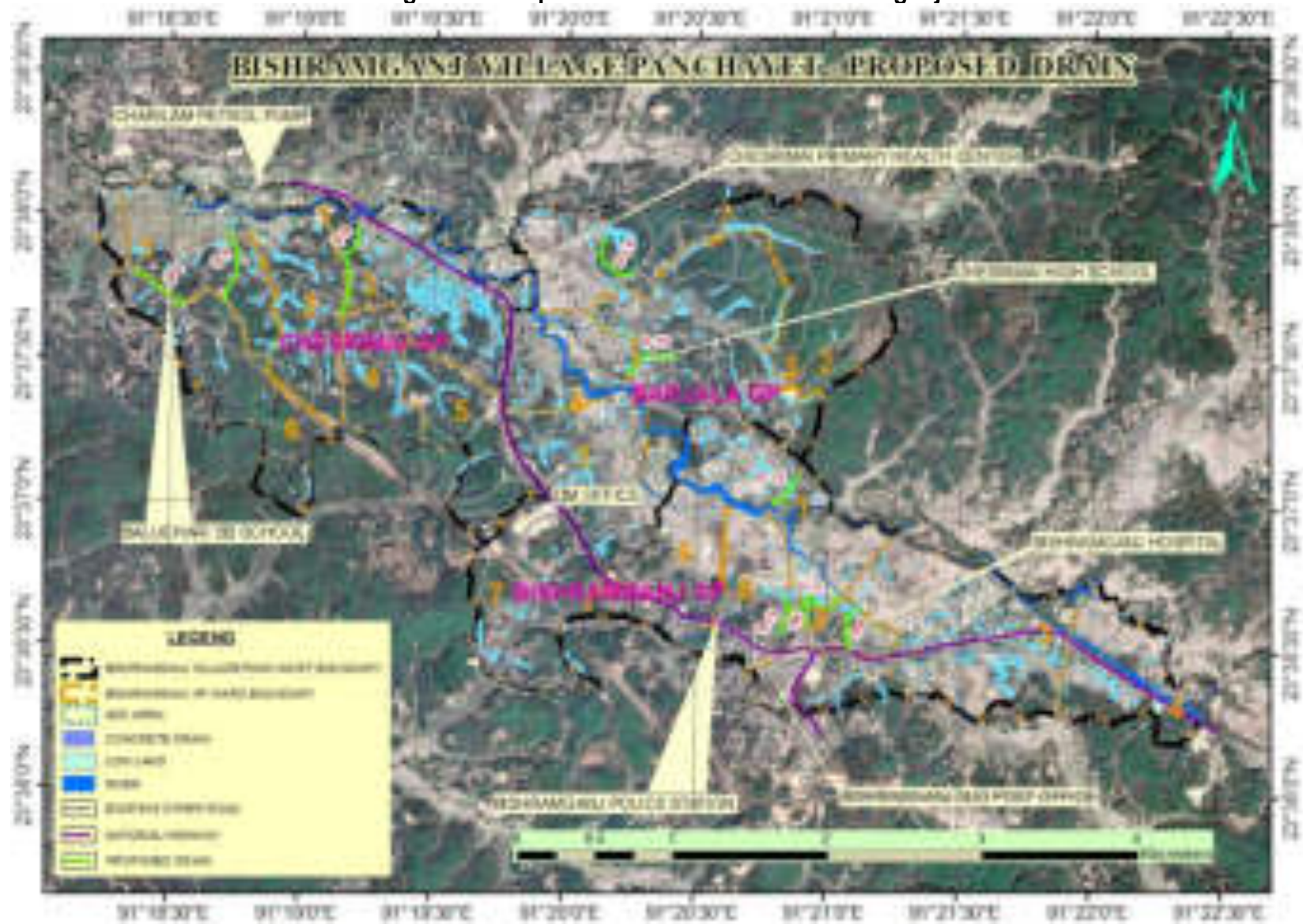
Figure 20: Proposed Drain network at Bishramganj
