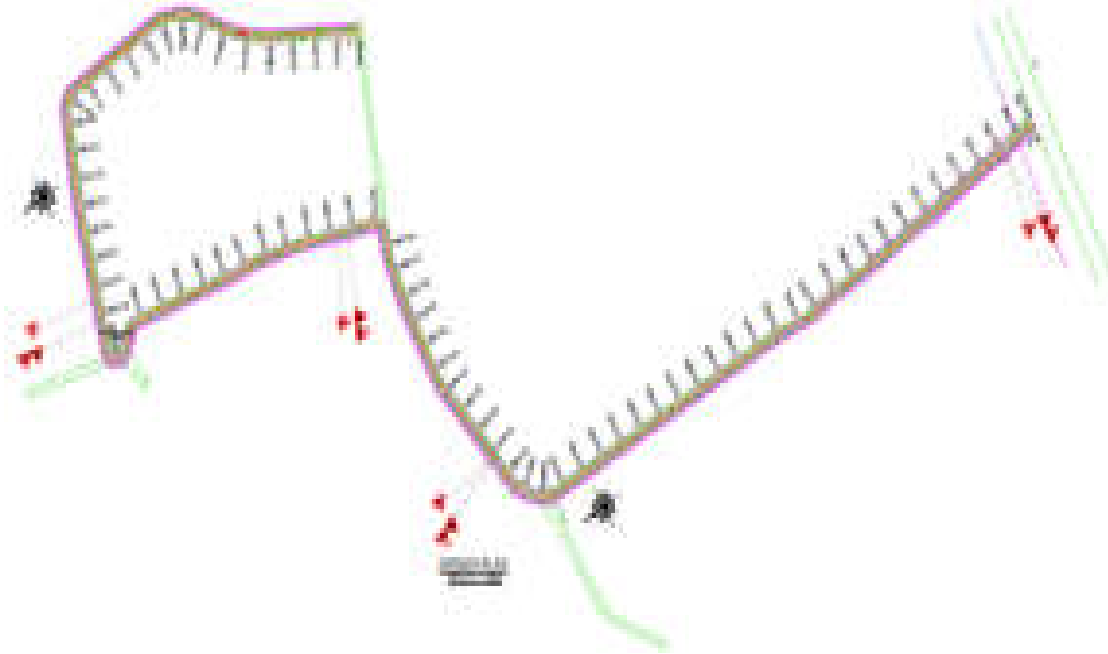
Figure 28: Proposed plan and Profile of the Roads of Belonia
