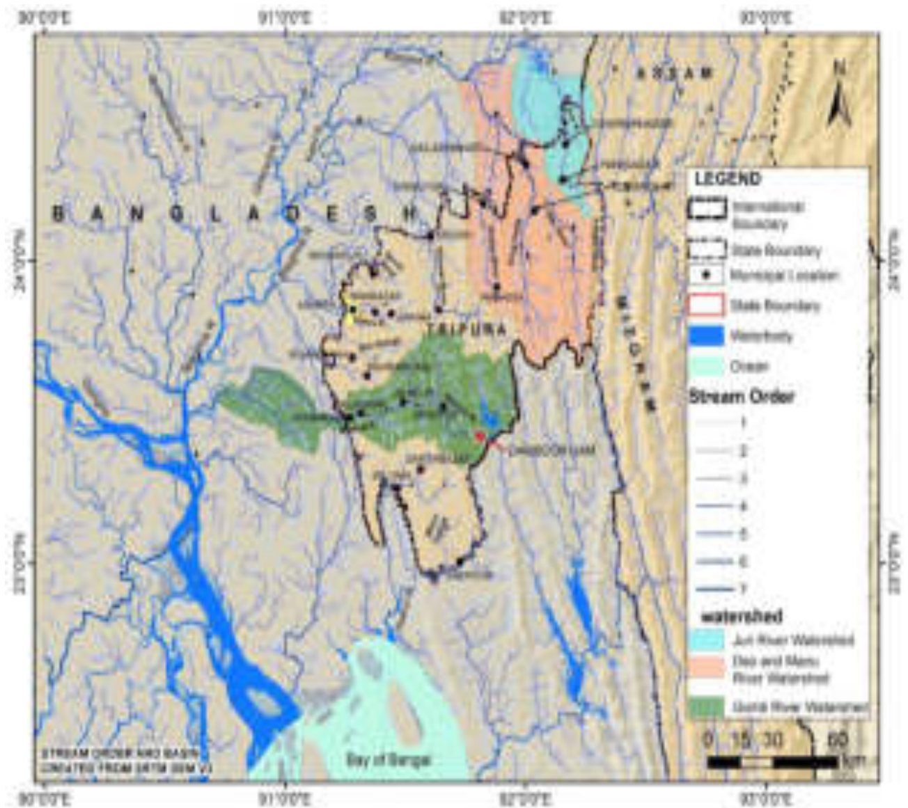
Figure 34: Watershed Map of Tripura watershed showing important rivers and Bangladesh International Boarder
