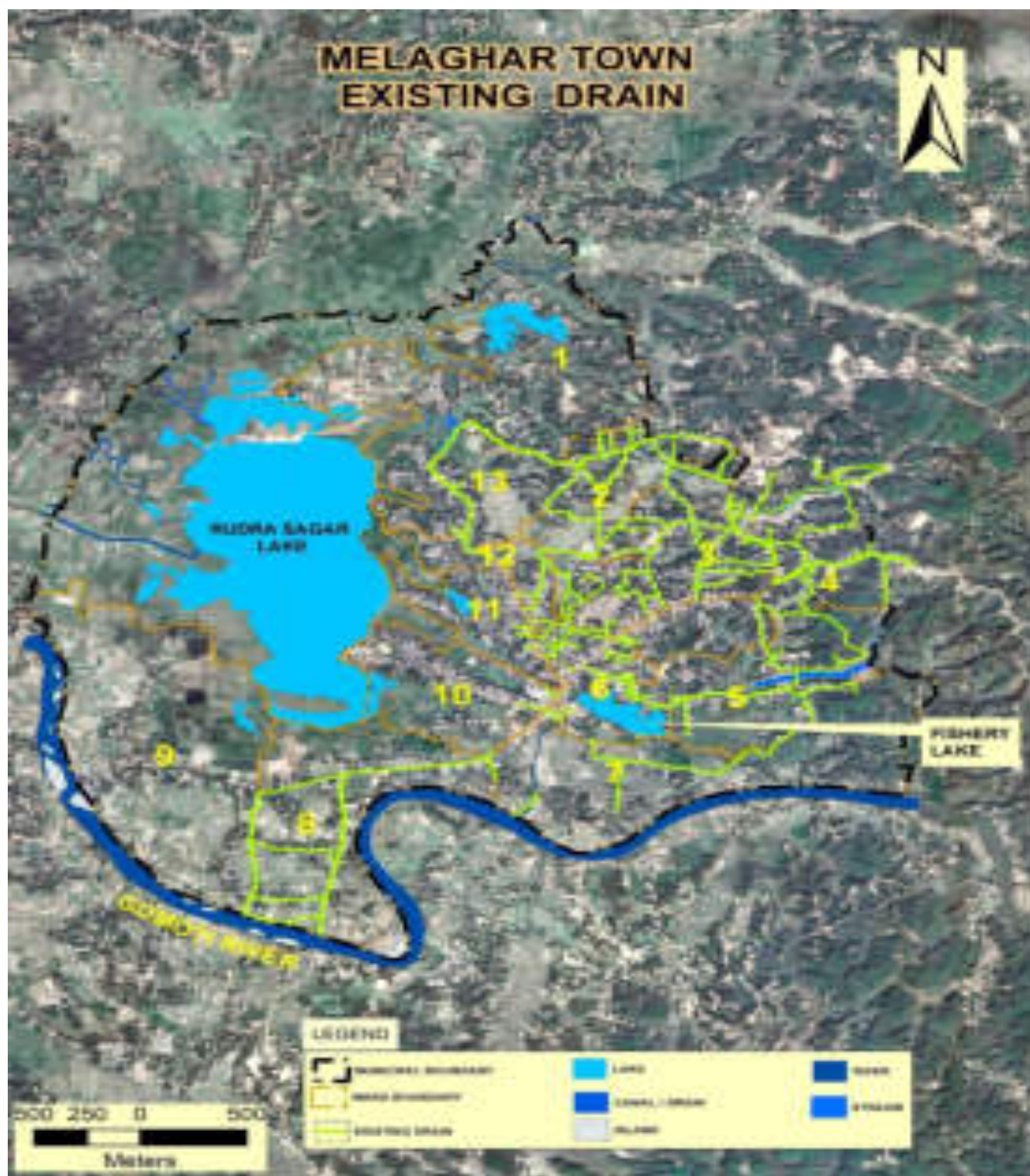
Figure 24: Existing Drainage network in Melaghar on google earth
