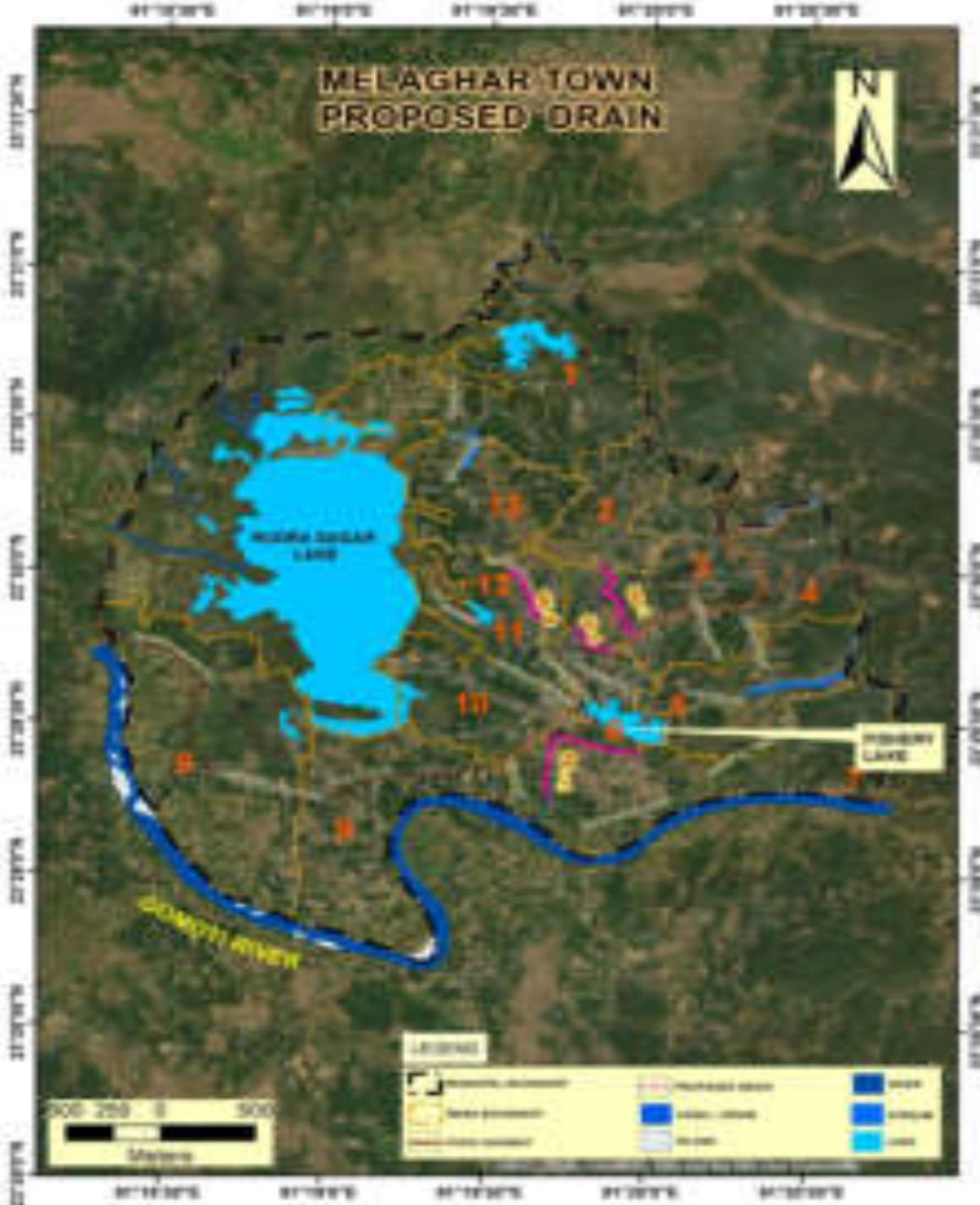
Figure 54: Proposed drains in Melaghar (pink) nearby Rudrasagar lake
